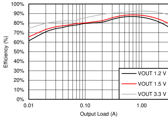
Figure 7-1. BUCK1 Efficiency
