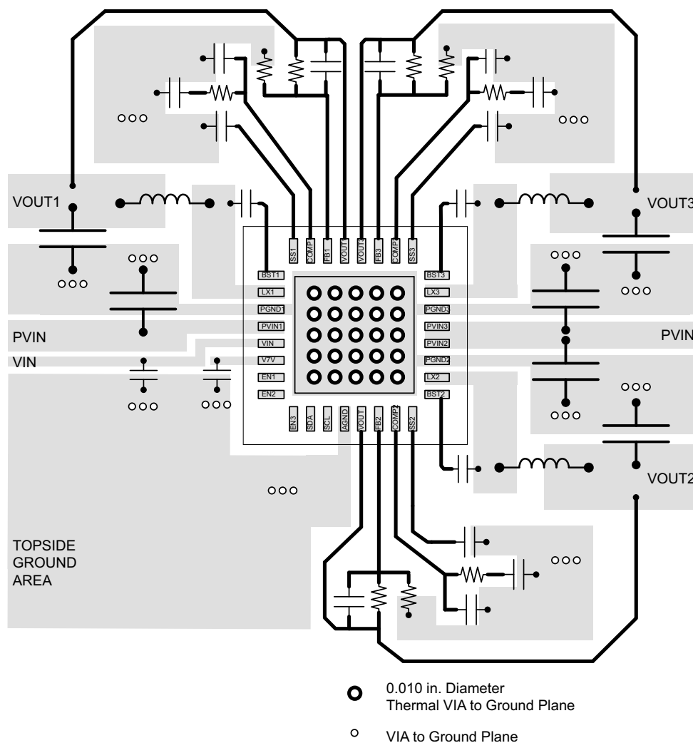
Figure 9-26. PCB Layout
