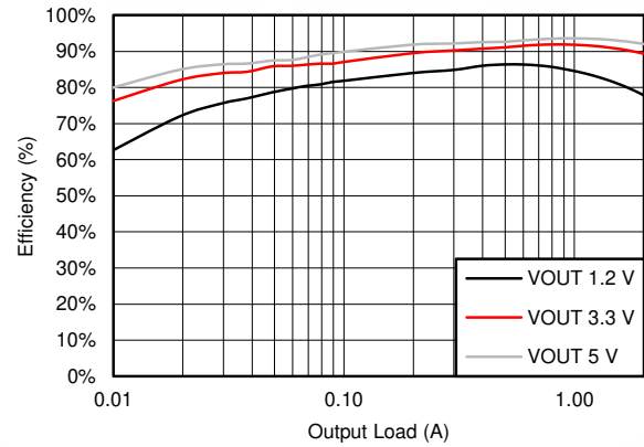
Figure 7-2. BUCK2 Efficiency
