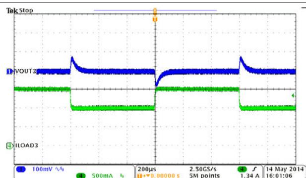
Figure 9-13. BUCK3, Load Transient, 1 to 1.5 A SR = 0.25 A/µs
