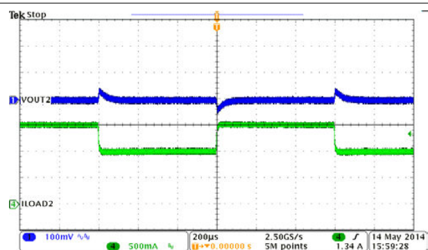
Figure 9-11. BUCK2, Load Transient, 1 to 1.5 A SR = 0.25 A/µs
