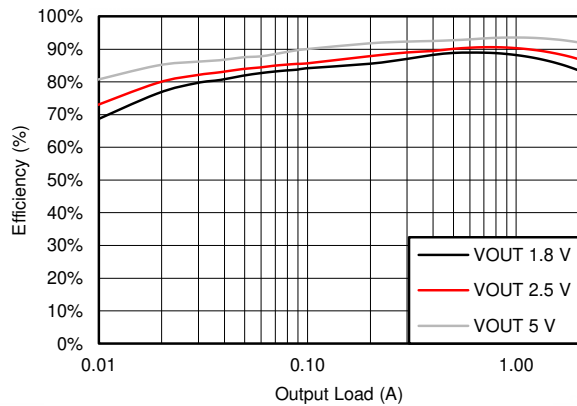
Figure 7-3. BUCK3 Efficiency
