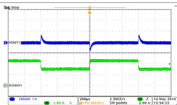
Figure 9-9. BUCK1, Load Transient, 1.5 to 2.25 A SR = 0.25 A/µs
