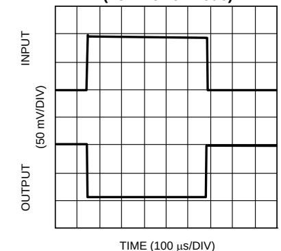
Small Signal Inverting Pulse Response (Low Power Mode)
