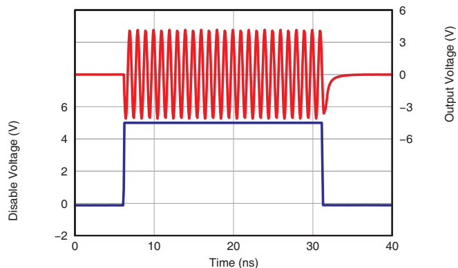
LARGE-SIGNAL ENABLE/DISABLE RESPONSE
