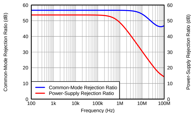
COMMON-MODE REJECTION RATIO AND POWER-SUPPLY REJECTION RATIO
