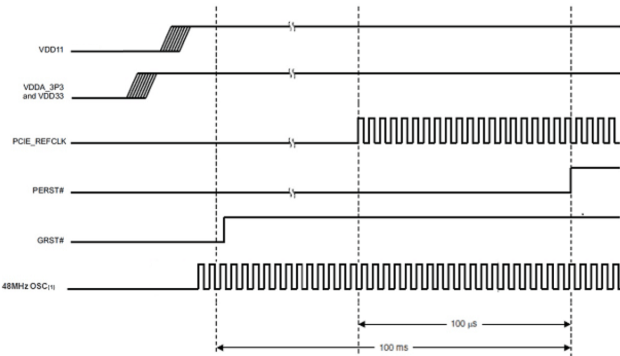
Figure 7-16. Power-Up Sequence
