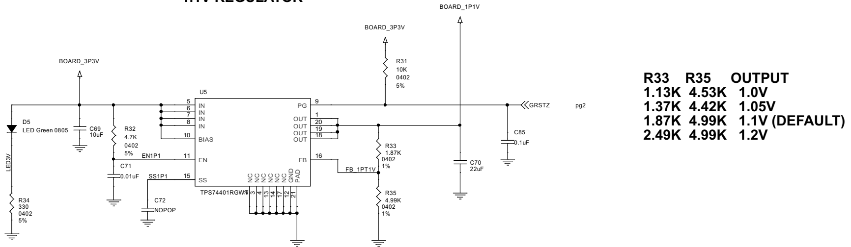
Figure 7-6. Reference Design 4
