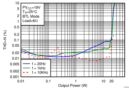
Figure 6-43. THD+N vs Output Power
