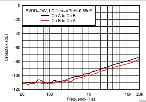
Figure 6-26. Crosstalk
