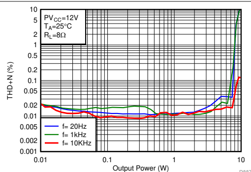
Figure 6-20. THD+N vs Output Power-BTL
