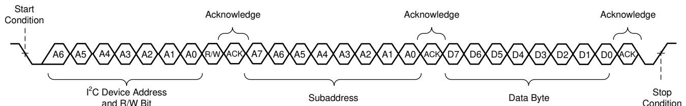
Figure 7-10. Random Write Transfer
