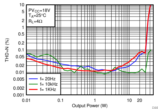
Figure 8-11. THD+N vs Output Power (Inductor as Output Filter, Hybrid Modulation, PBTL mode)
