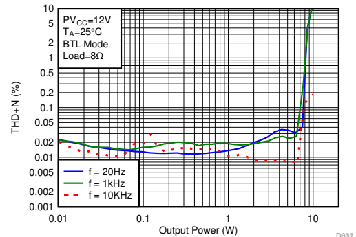
Figure 6-44. THD+N vs Output Power
