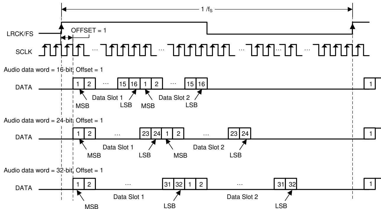
Figure 7-5. TDM 1 Audio Data Format
