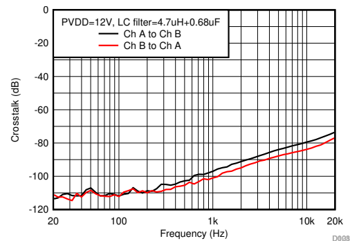
Figure 6-26. Crosstalk
