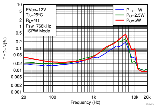
Figure 6-1. THD+N vs Frequency-BTL
