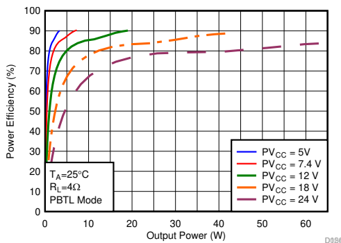
Figure 8-10. Efficiency vs Output Power (Inductor as Output Filter, Hybrid modulation, PBTL mode)
