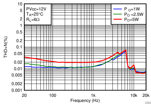
Figure 6-4. THD+N vs Frequency-BTL
