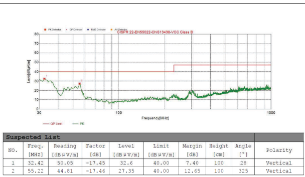
Figure 8-8. Radiated Emission with Ferrite Bead Filter - Vertical
