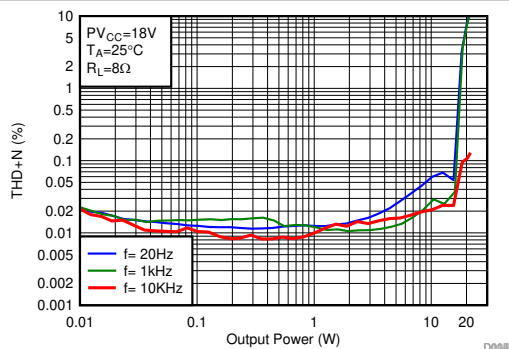
Figure 6-21. THD+N vs Output Power-BTL
