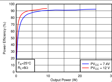
Figure 6-64. Efficiency vs Output Power-BTL
