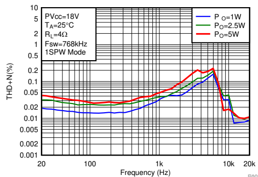
Figure 6-2. THD+N vs Frequency-BTL
