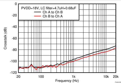
Figure 6-28. Crosstalk
