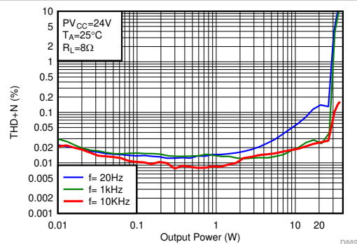
Figure 6-22. THD+N vs Output Power-BTL
