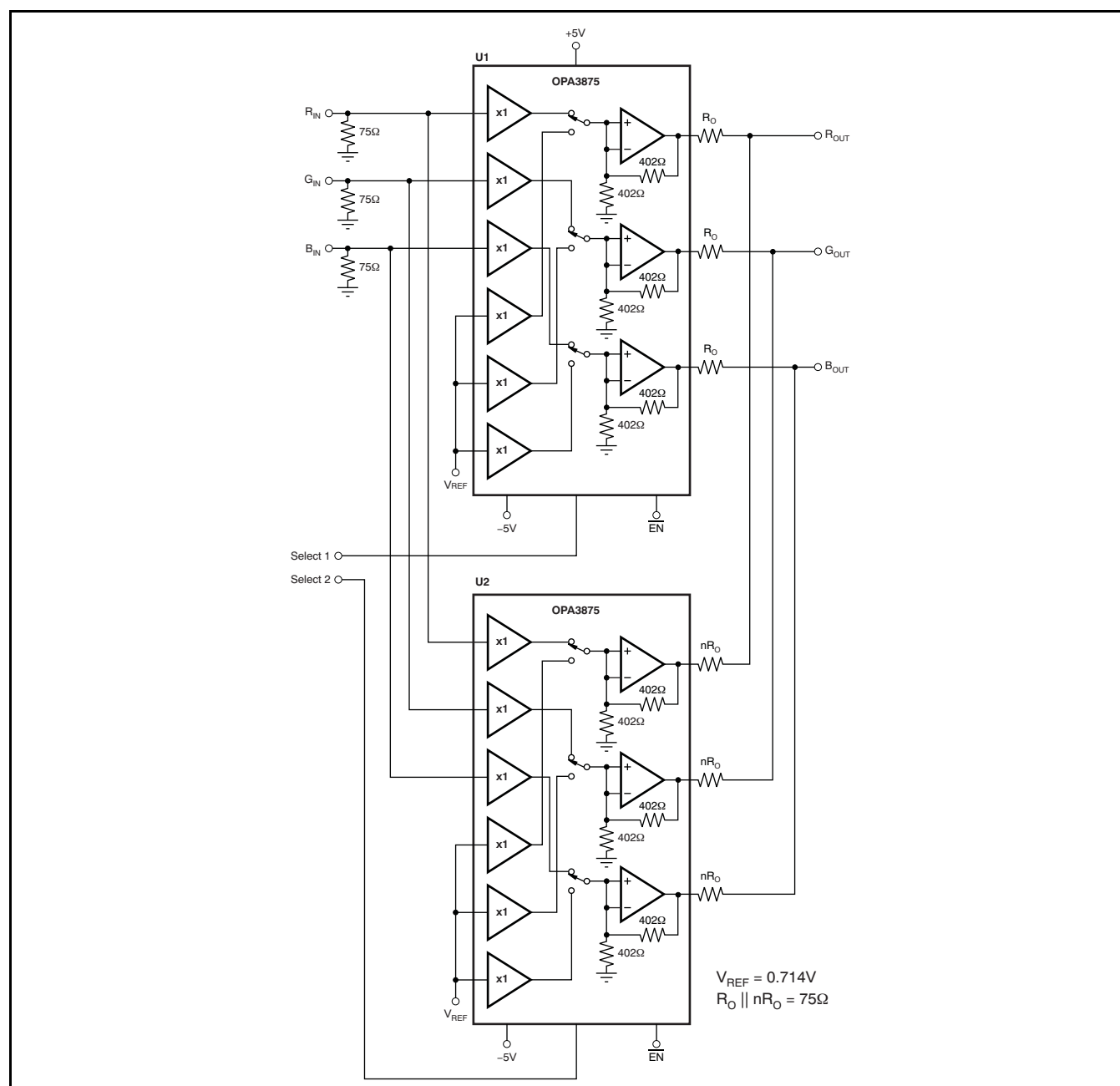
Figure 28. Logo Inserter
