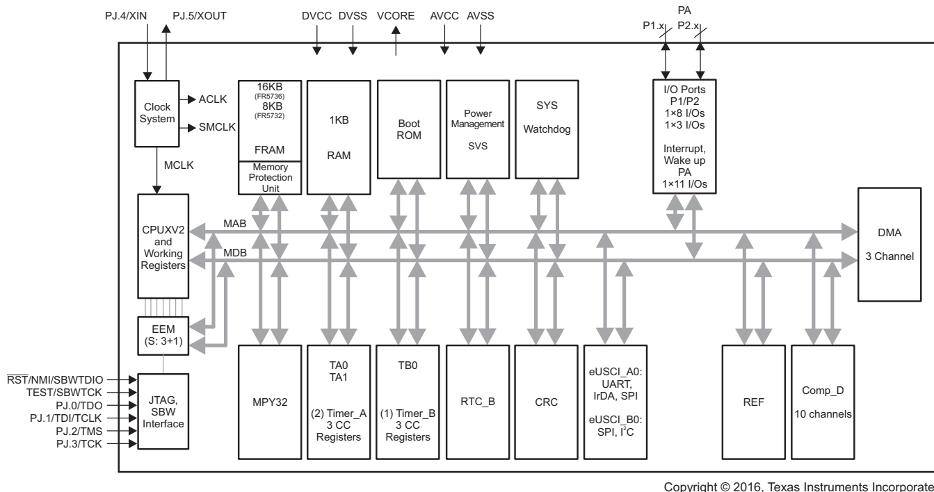
Figure 6-6. Functional Block Diagram – RGE Package – MSP430FR5732, MSP430FR5736
