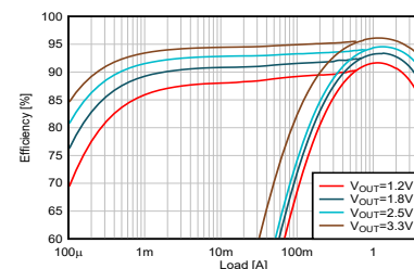
Efficiency at V_{IN} = 5V
