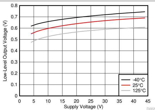
Figure 6-2. V_{OL} vs V_{SUP} and Temperature
