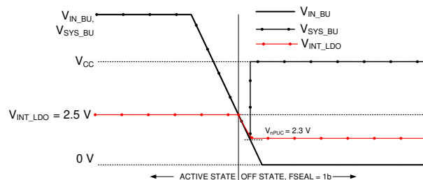
Figure 8-18. Switching Behavior of the Battery-Backup-Supply Power-Path; Main Power Supply Removal
