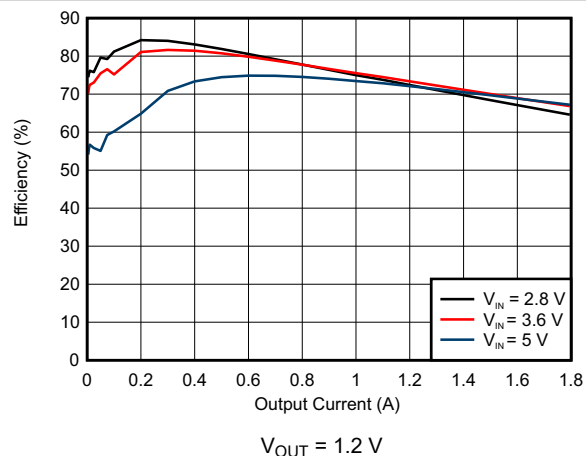
Figure 9-5. DCDC3 Efficiency
