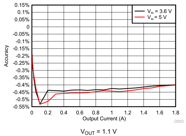
Figure 7-2. DCDC2 Accuracy
