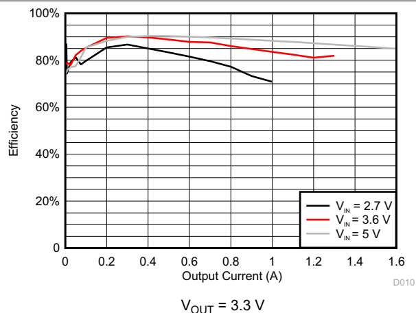
Figure 9-7. DCDC4 Efficiency
