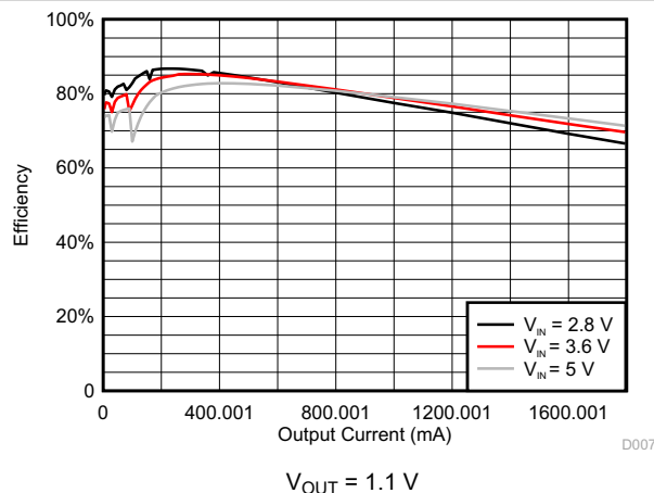
Figure 9-4. DCDC1/DCDC2 Efficiency
