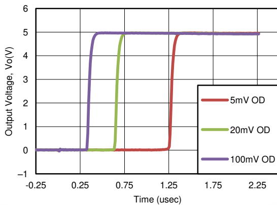
Figure 7-2. Response Time for Various Overdrives (Positive Transition)
