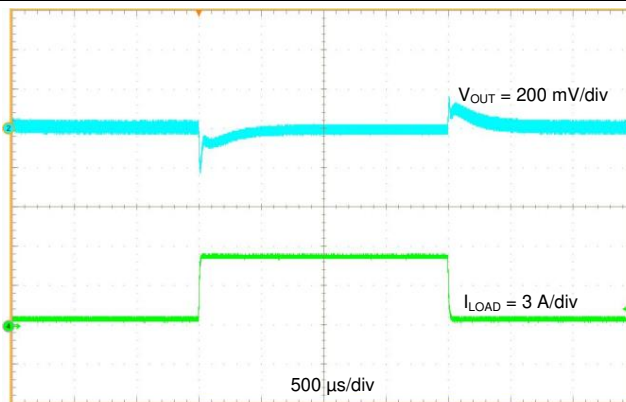
Figure 26. Transient Response 0 to 3 A
