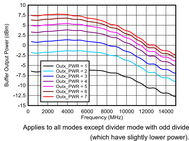
Figure 5-9. Buffer Mode Single-Ended Output Power
