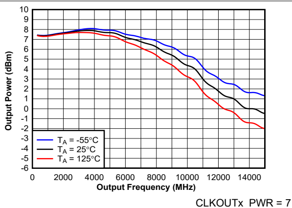
Figure 5-10. Buffer Mode Single-Ended Output Power
