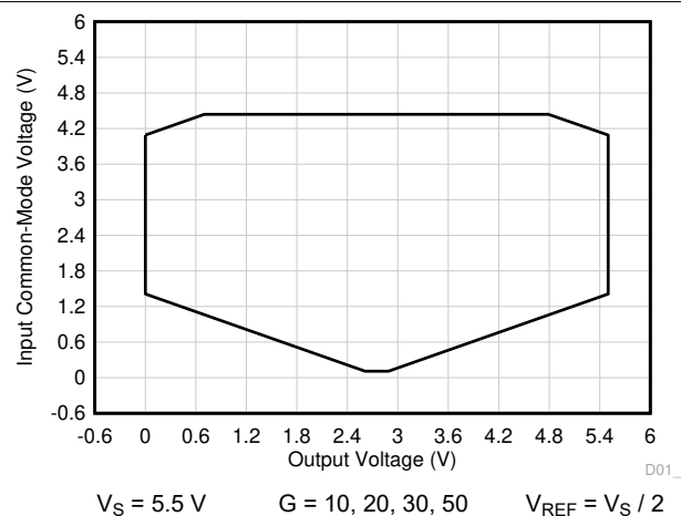
Figure 7-53. Input Common-Mode Voltage vs Output Voltage (High CMRR Region)
