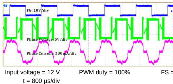
Figure 1. Start Up at 100% Duty
