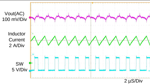
Figure 14. Switching Waveforms in CCM
