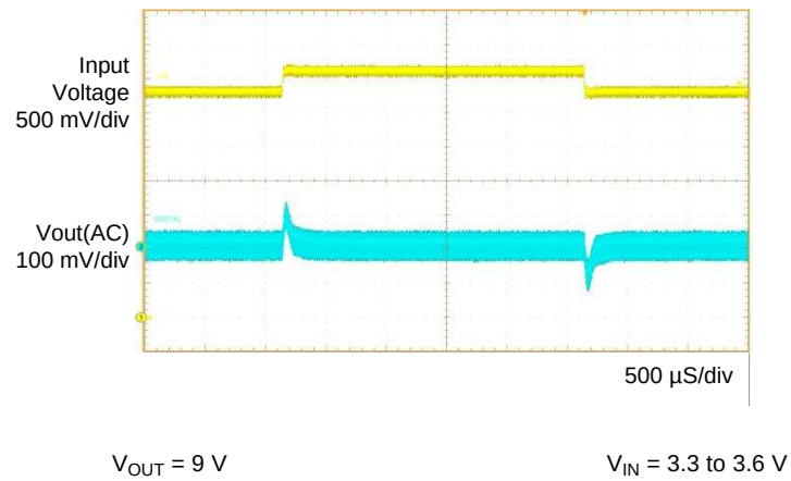
Figure 20. Line Transient
