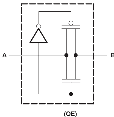
Figure 6. Simple Schematic
