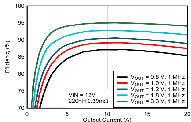
Typical Application Efficiency
