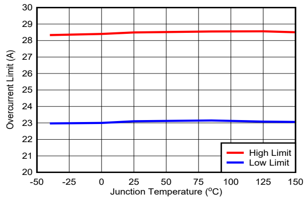
Figure 5-3. Overcurrent Limit
