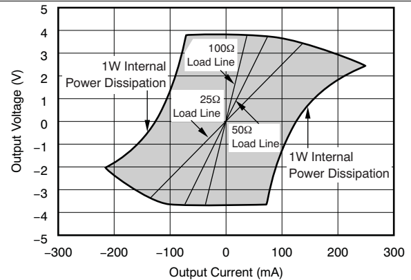
Figure 46. Output Voltage and Current Limitations
