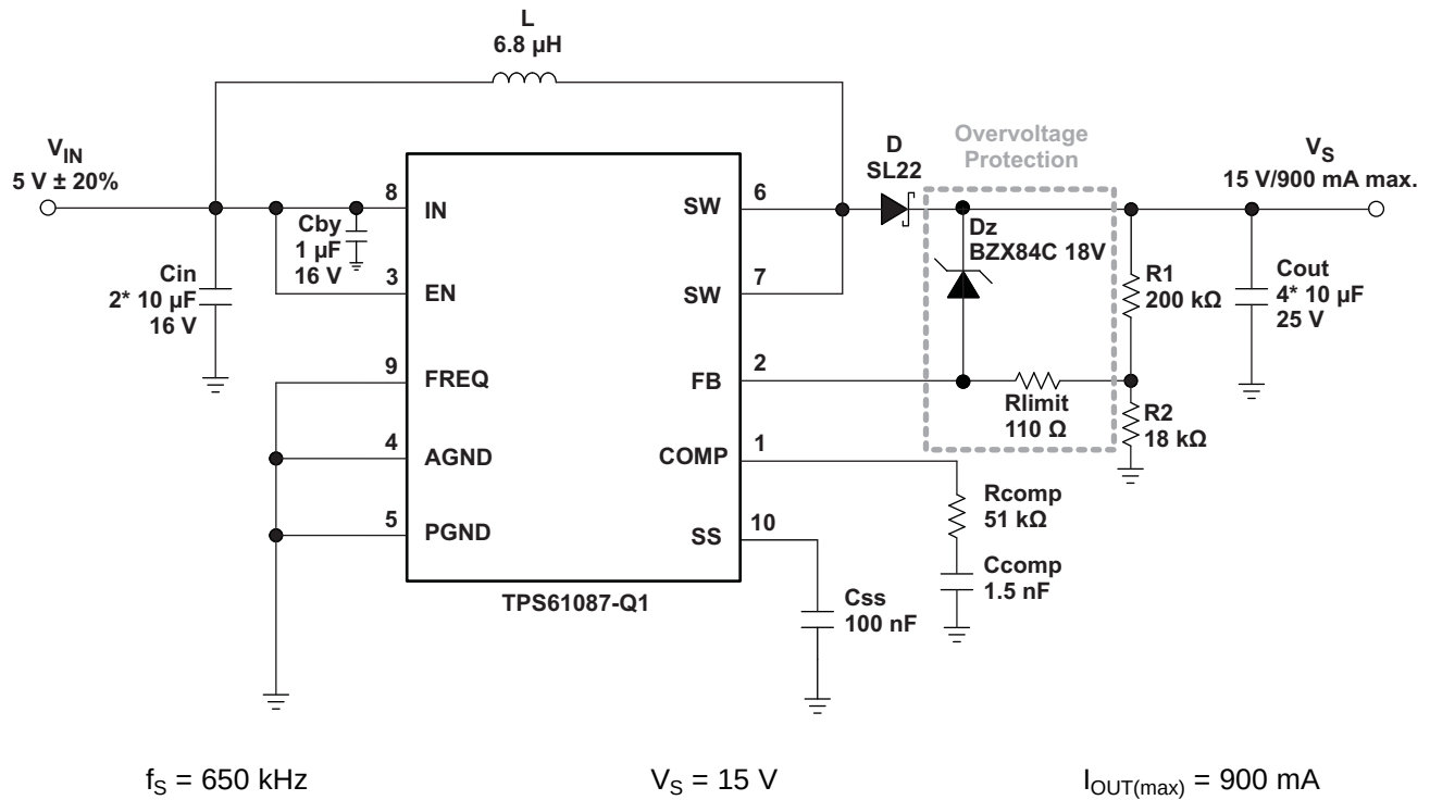
Figure 18. Application Diagram for 5 V to 15 V With Overvoltage Protection
