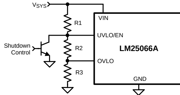
Figure 35. Shutdown Control
