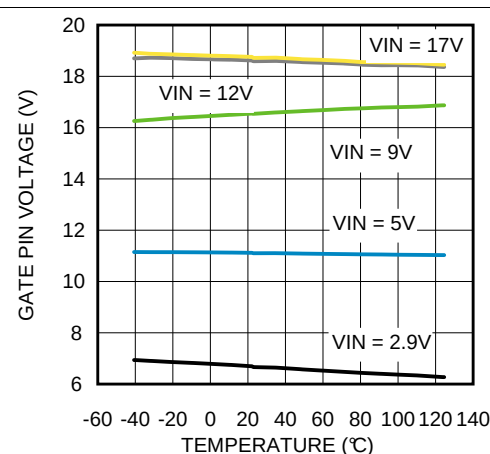
Figure 7. GATE Pin Voltage
