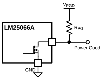
Figure 44. Power Good Output
