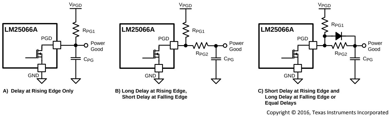
Figure 45. Adding Delay to the Power Good Output Pin
