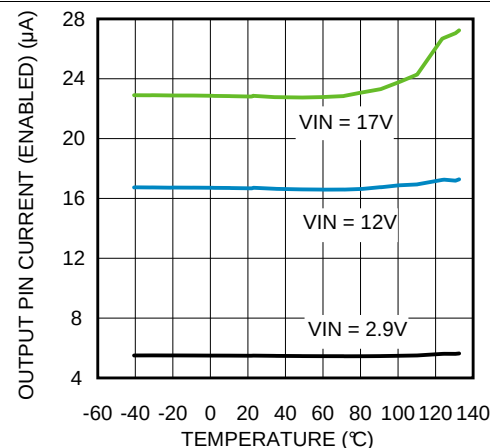
Figure 5. OUT Pin Current (Enabled)
