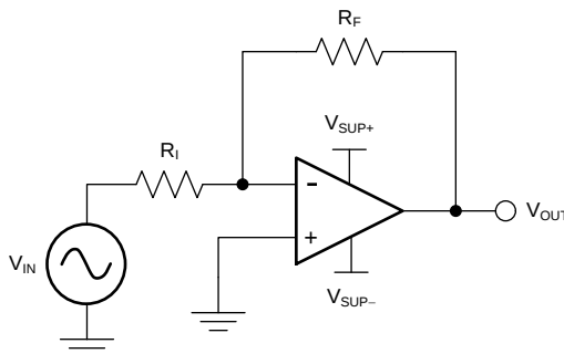
Figure 28. Application Schematic
