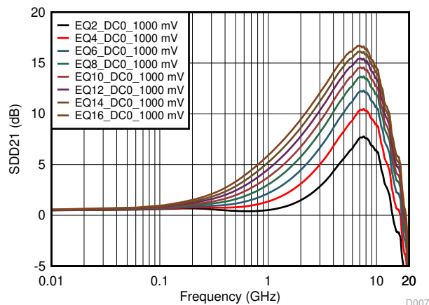
Figure 5-7. 1000mV DC0 Gain Even EQ Settings Curves
