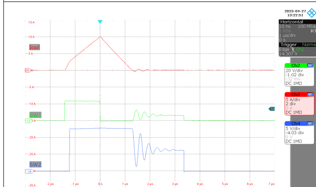
Figure 8-8. Inductor current buck operation (MODE = 0 V, V_o = 12 V, I_o = 10 mA, V_{(VIN)} = 24 V)
