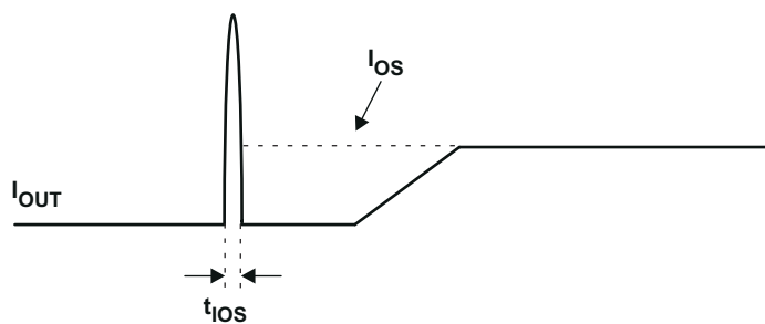
Figure 7-2. Response Time to Short-Circuit Waveform
