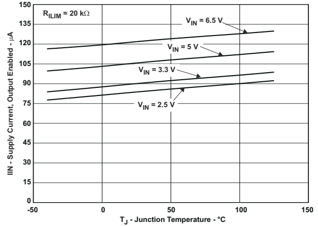
Figure 6-14. I_{IN} – Supply Current, Output Enabled – \mu A
