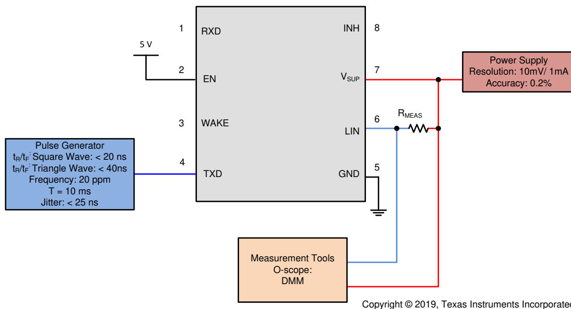
Figure 8-6. Test Circuit for I_{\text{BUS\_LIM}} at Dominant State (Driver on) Param 12
