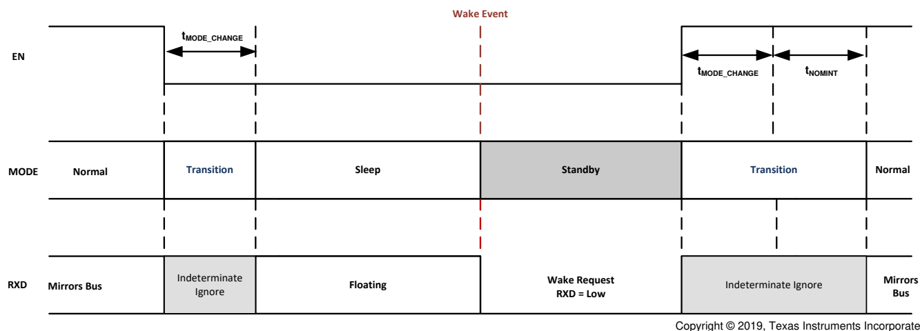
Figure 8-14. Mode Transitions
