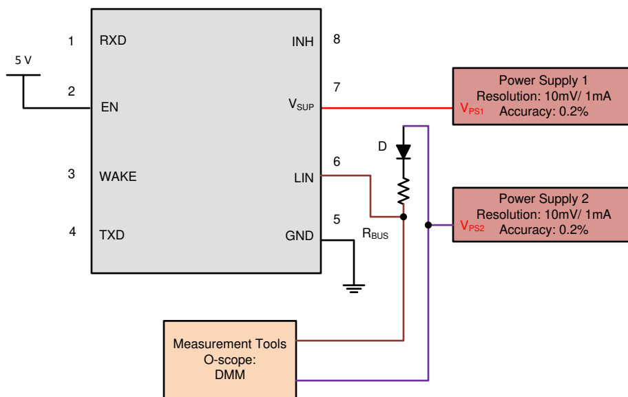
Figure 8-4. LIN Receiver Test with RX access Param 17, 18, 19, 20
