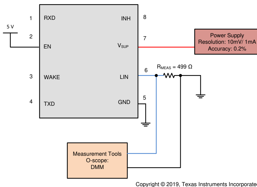
Figure 8-7. Test Circuit for I_{\text{BUS\_PAS\_dom}} ; TXD = Recessive State V_{\text{BUS}} = 0 \text{ V} , Param 13
