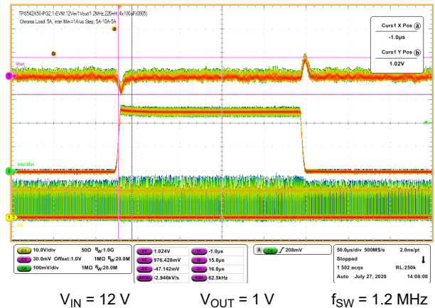
Figure 8-3. Load Transient 5 A to 10 A to 5 A at 1 A/ \mu s
