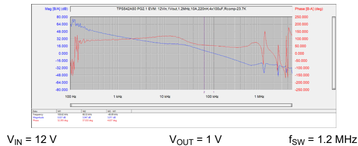
Figure 8-4. Bode Plot at 10-A Output Current
