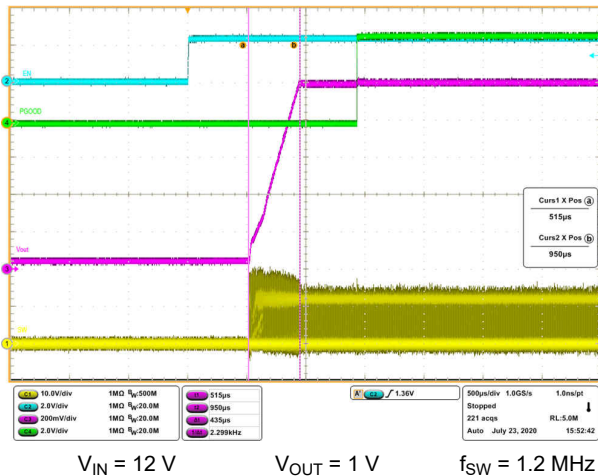
Figure 8-2. 450 \mu s Start-up by EN at 0-A Output Current
