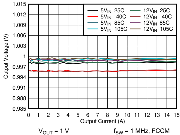
Figure 6-7. Load Regulation
