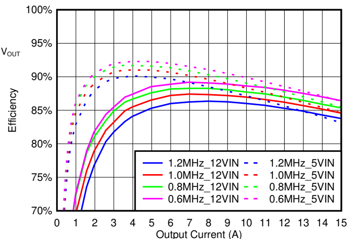
Typical Efficiency at 1 V OUT
