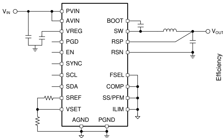
Simplified Schematic
