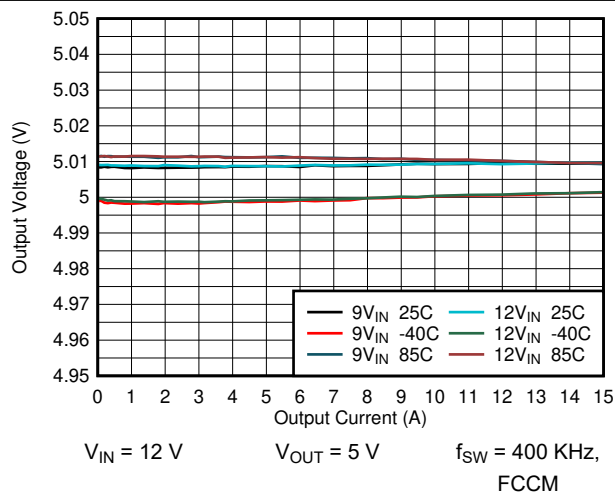
Figure 6-9. Load Regulation
