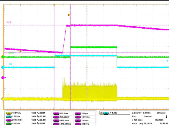
Figure 6-18. 50% Pre-biased Start-up by EN at 0-A Output Current
