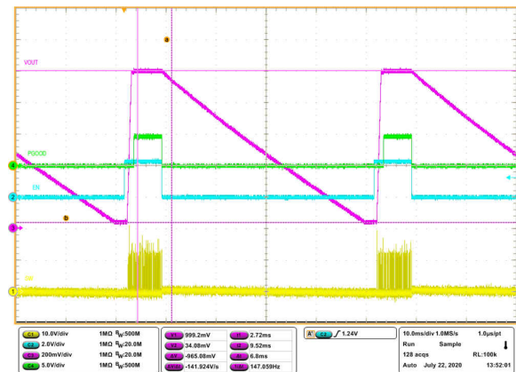
Figure 6-19. Start-up and Shutdown by EN at 0-A Output Current
