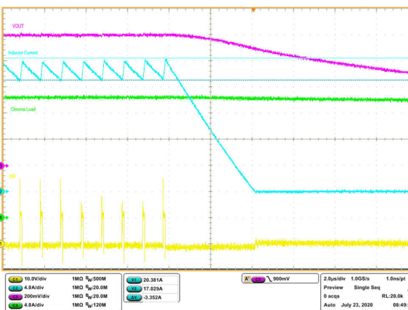
Figure 6-23. 20-A Overcurrent Protection by Electronic Load
