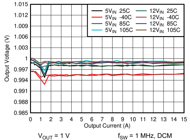
Figure 6-8. Load Regulation
