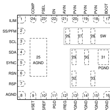
Figure 5-1. 33-Pin VQFN RJM Package (Top View)
