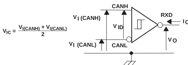
Figure 6. Receiver Voltage and Current Definitions
