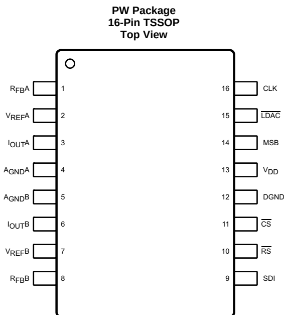
Pin Functions
