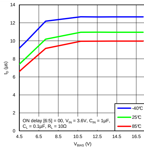
Figure 18. t_D vs. V_{BIAS} (ON delay [6:5] = 00)
