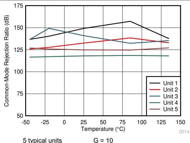
Figure 7-15. CMRR vs Temperature
