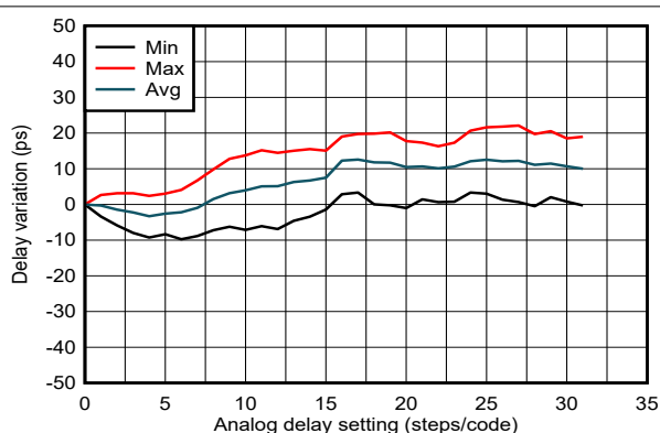
Figure 6-23. SYSREF/1PPS Delay Linearity vs. Analog Delay Code 5
