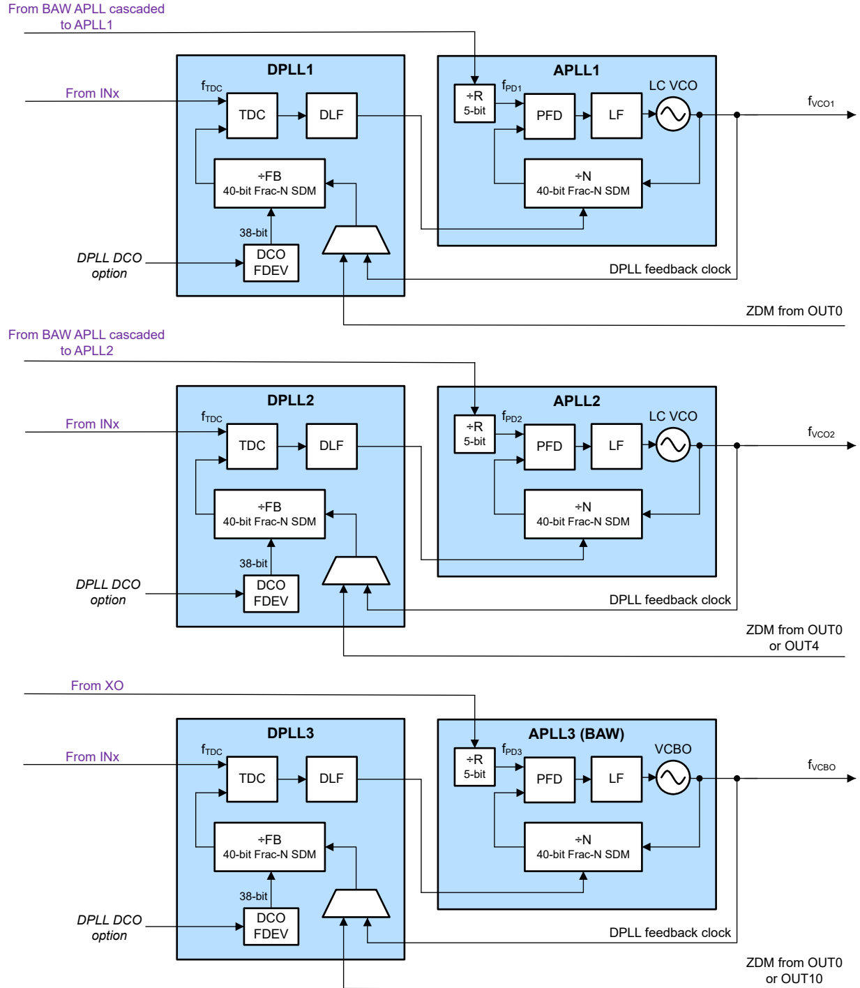
Figure 8-5. APLL Cascaded With DPLLs Enabled Example
