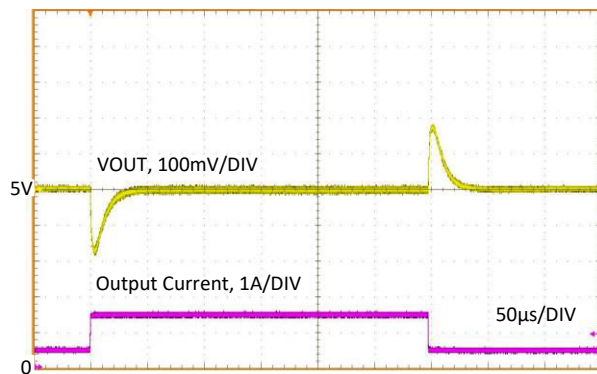
LM63615 V_{OUT} = 5V f_{SW} = 2100kHz 0.5A to 1.5A, 2µs AUTO
