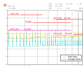
Figure 9-64. LM73606-Q1 Conducted EMI Result versus CISPR25 Limits - High Frequency
