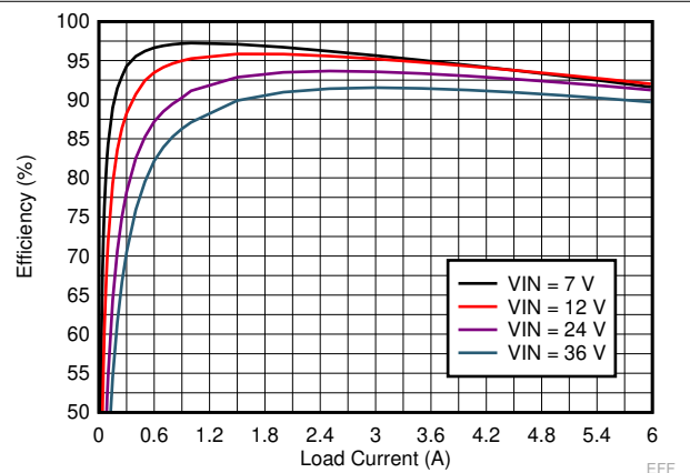
Figure 9-12. LM73606-Q1 Efficiency
