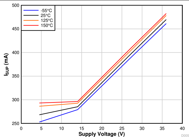
Figure 7-4. I_{SUP} Recessive vs V_{SUP} and Temperature
