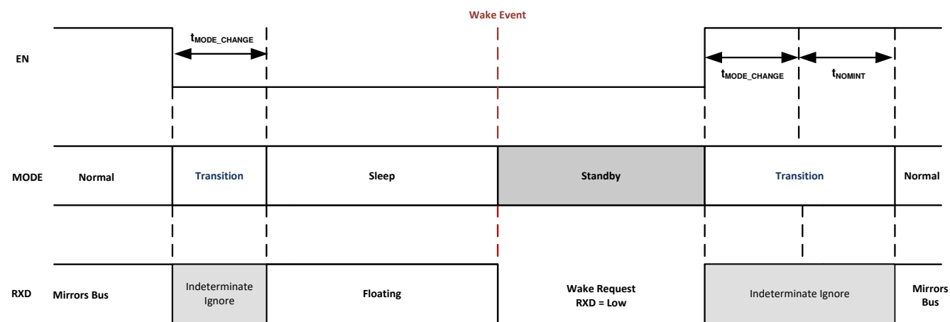
Figure 8-15. Mode Transitions
