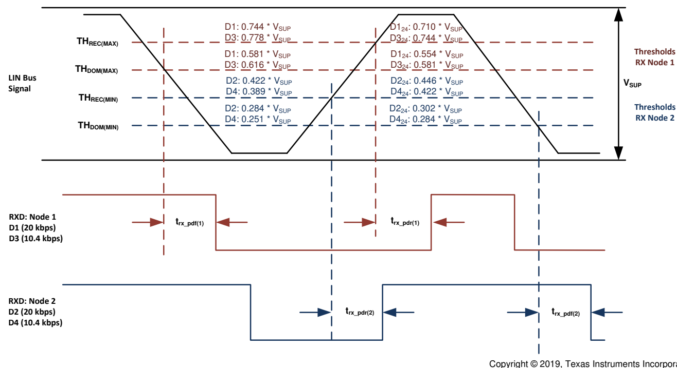
Figure 8-14. Propagation Delay
