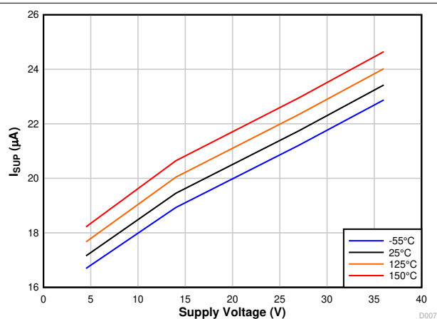
Figure 7-6. Standby Mode I_{SUP} Recessive vs V_{SUP} and Temperature
