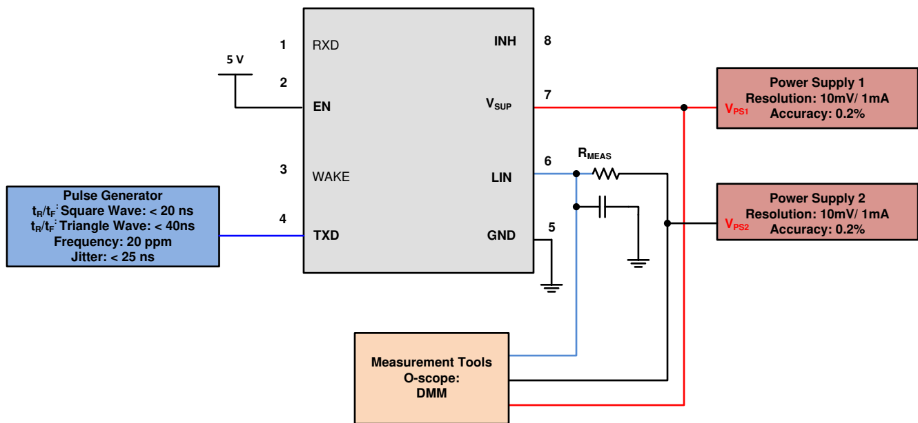
Figure 8-11. Test Circuit Slope Control and Duty Cycle Param 27, 28, 29, 30
