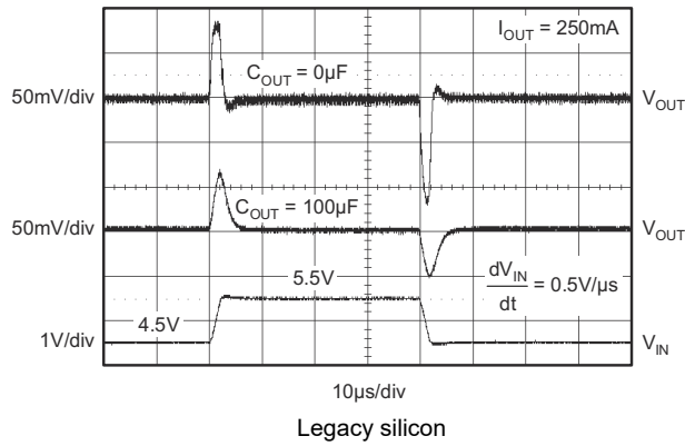
Figure 5-37. TPS73233-Q1 – Line Transient Response
