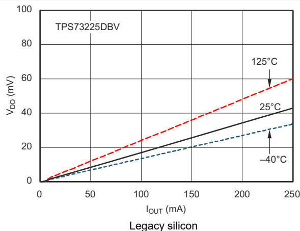
Figure 5-5. Dropout Voltage vs Output Current
