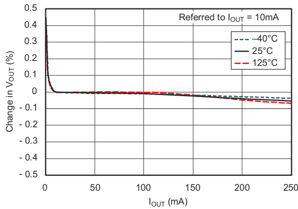
Figure 5-1. Load Regulation
