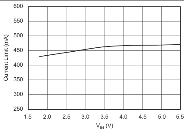
Legacy silicon Figure 5-19. Current Limit vs V_{IN}
