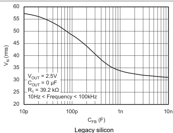
Figure 5-47. TPS73201-Q1 – RMS Noise Voltage vs C_{ADJ}
