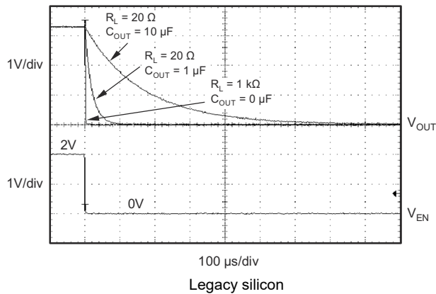
Figure 5-41. TPS73233-Q1 – Turnoff Response
