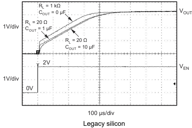
Figure 5-39. TPS73233-Q1 – Turnon Response
