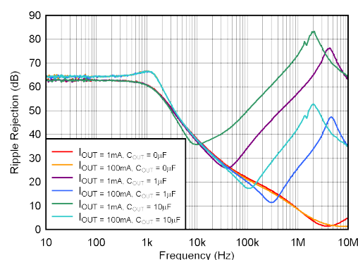
New silicon Figure 5-24. PSRR (Ripple Rejection) vs Frequency
