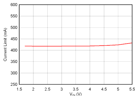
New silicon Figure 5-20. Current Limit vs V_{IN}
