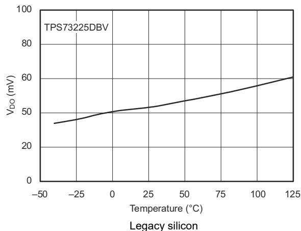
Figure 5-7. Dropout Voltage vs Temperature
