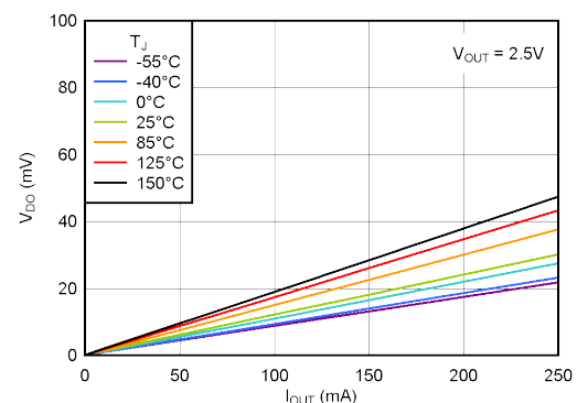
Figure 5-6. Dropout Voltage vs Output Current
