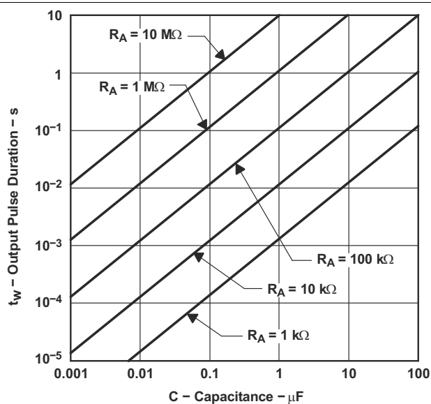
Figure 6-4. Output Pulse Duration vs Capacitance
