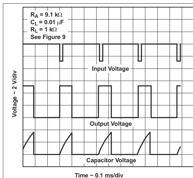
Figure 6-3. Typical Monostable Waveforms
