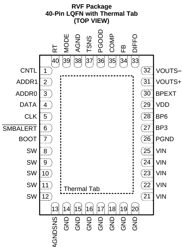
Pin Functions
