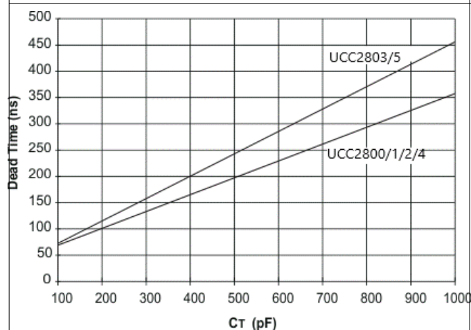
Figure 6-9. Dead Time vs C_T , R_T = 100\text{ k}
