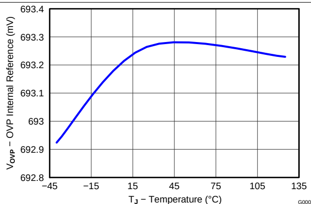
Figure 13. OVP Internal Reference vs Temperature
