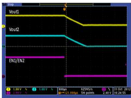
Figure 22. Shutdown With Enable
