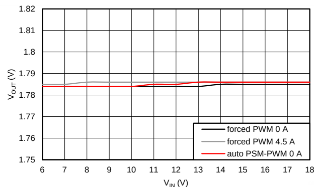
Figure 15. 1.8-V Line Regulation V_{OUT} = 1.8\text{ V}
