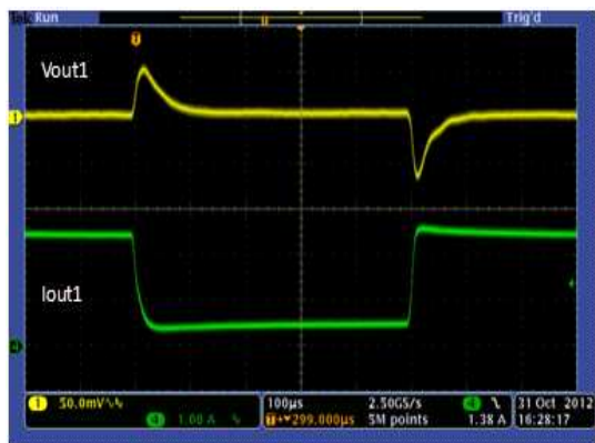
Figure 24. Load Transient, Buck 1 (0.5 A - 2.5 A)
