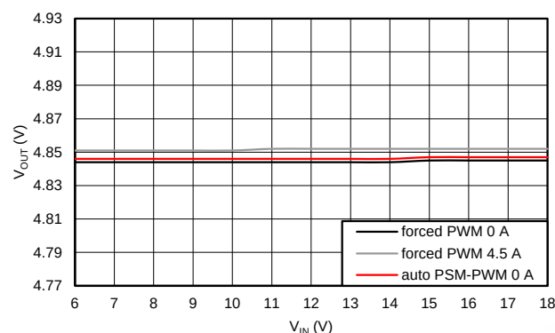
Figure 17. 5-V Line Regulation V_{OUT} = 5\text{ V}
