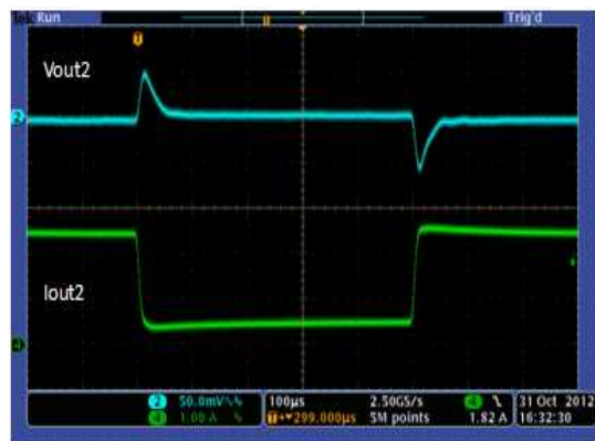
Figure 25. Load Transient, Buck 2 (0.5 A - 2.5 A)
