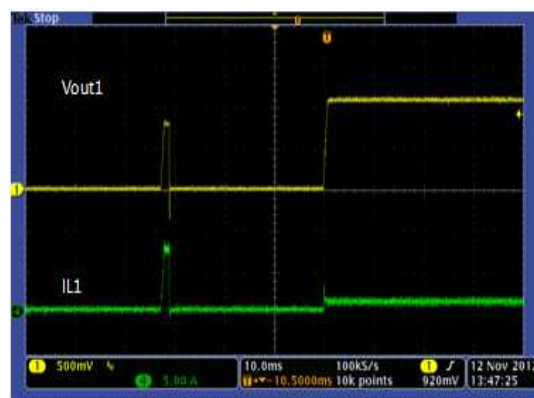
Figure 27. Hiccup Recover, Buck 1
