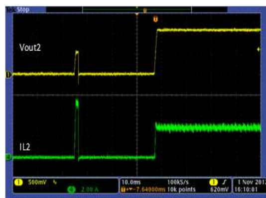
Figure 29. Hiccup Recover, Buck 2
