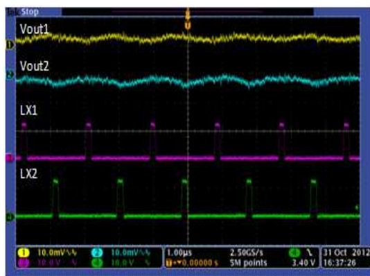
Figure 18. Output Ripple at 0 A, Forced PWM
