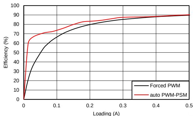
Figure 7. 3.3-V Efficiency, Light Load V_{IN} = 12\text{ V} , V_{OUT} = 3.3\text{ V}
