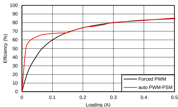
Figure 5. 1.8-V Efficiency, Light Load V_{IN} = 12\text{ V} , V_{OUT} = 1.8\text{ V}
