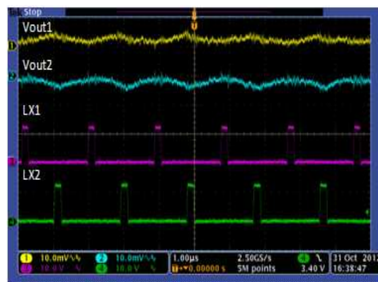
Figure 19. Output Ripple at 3.5 A, Forced PWM
