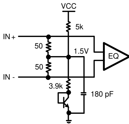
Figure 7-1. Receiver Input Termination and Bias Circuit
