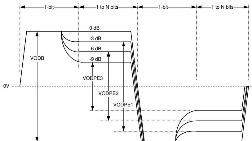
Figure 7-2. Driver Pre-Emphasis Differential Waveform (Showing All 4 Pre-Emphasis Steps)
