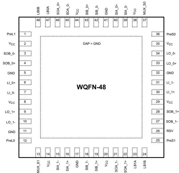
Figure 4-1. NJU Package 48-Pin WQFN Top View
