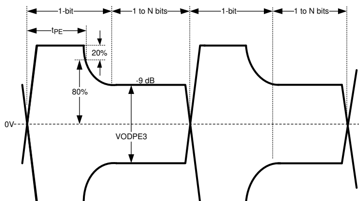
Figure 5-3. Test Condition for Output Pre-Emphasis Duration
