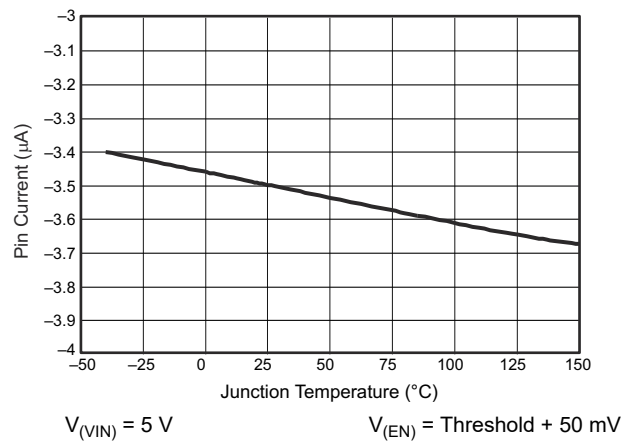
Figure 6-10. EN Pin Current vs Temperature
