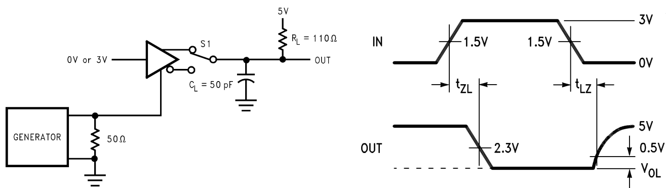
Figure 6. Driver Enable and Disable Times ( t_{ZL} , t_{LZ} , t_{LZL} ) (5)(6)(7)
