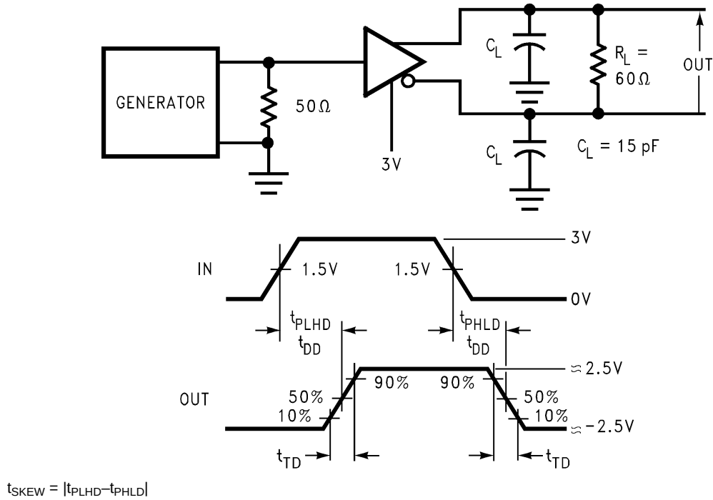
Figure 3. Driver Differential Output Delay and Transition Times (2)(3)
