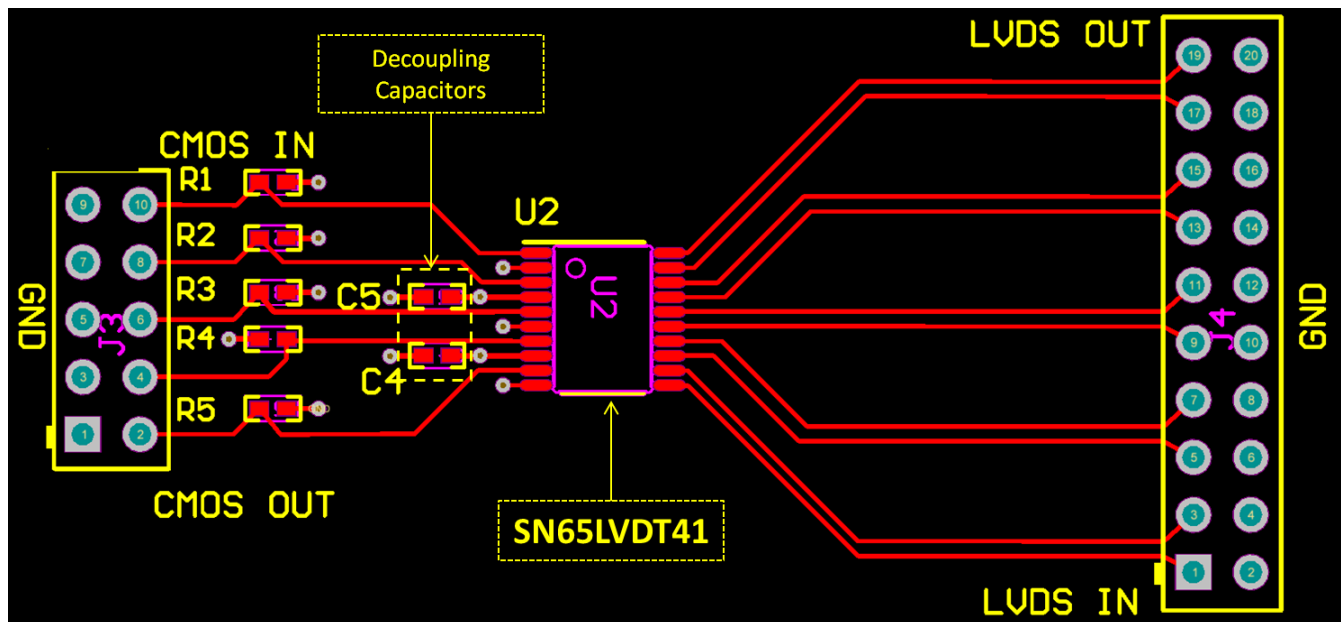
Figure 33. Example SN65LVDT41
