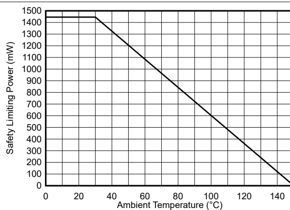
Figure 5-2. Thermal Derating Curve for Safety Limiting Power for Wide-SOIC (DW-16) Package
