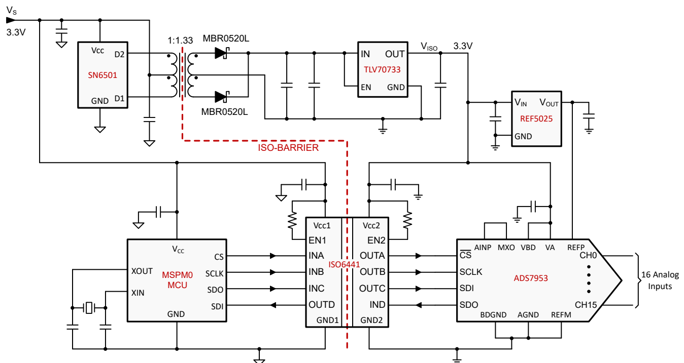
Figure 8-1. Isolated SPI for an Analog Input Module With 16 Inputs
