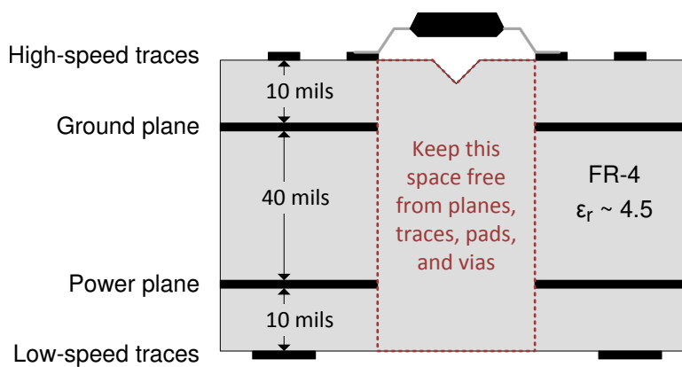
Figure 8-7. Layout Example PCB cross section
