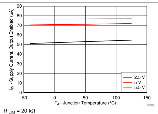
Figure 16. I_{IN} – Supply Current, Output Enabled – \mu\text{A}
