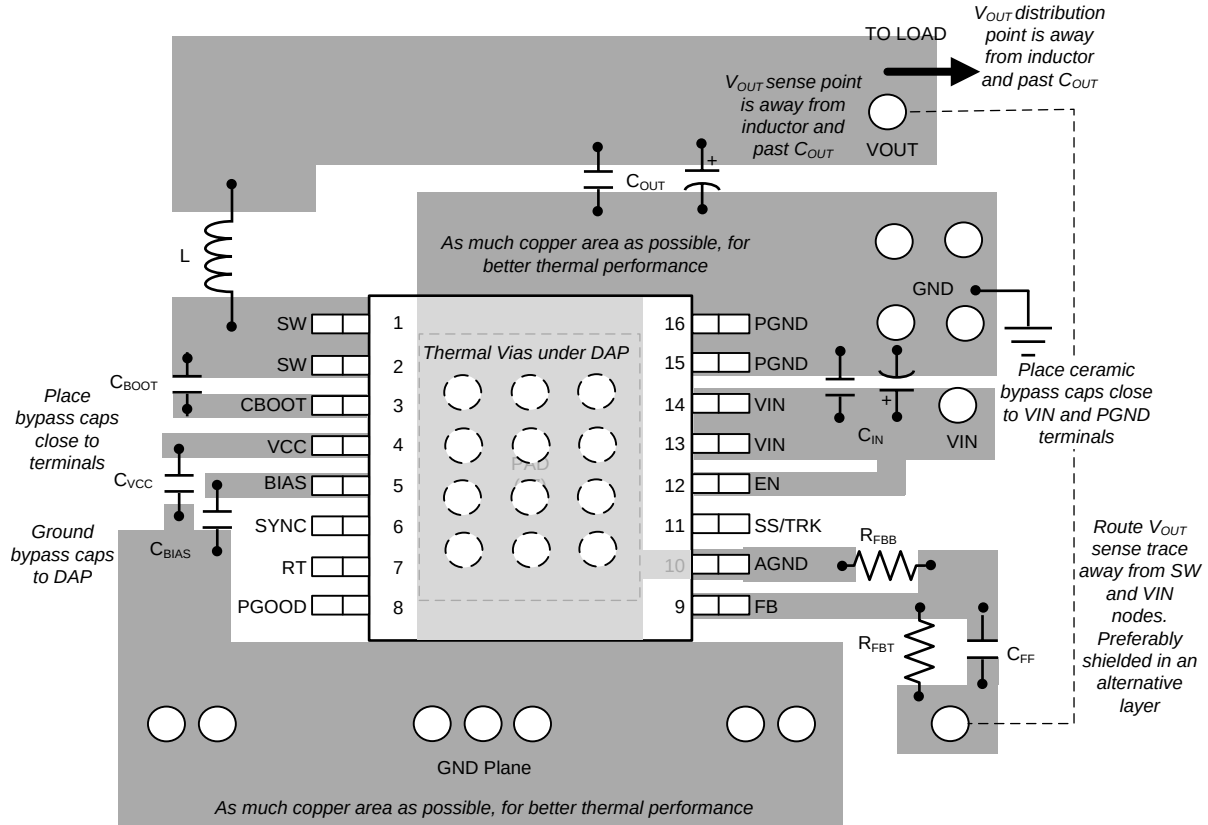
Figure 65. LM43602-Q1 Layout Example
