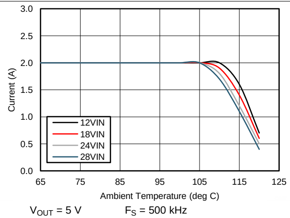
Figure 62. Derating Curve
