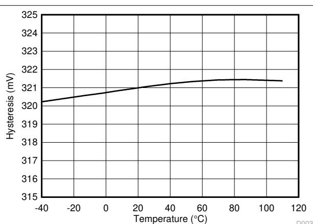
Figure 9-3. V_{HYS} vs Temperature
