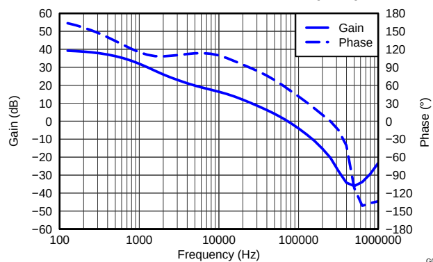
CLOSED LOOP RESPONSE, VIN (3.3 V), 4 A
