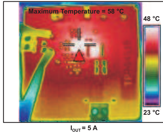
Figure 41. Thermal Image
